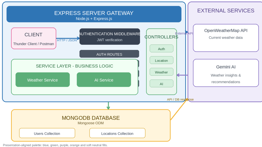
Figure 6.1: System Architecture of AI WeatherWise
